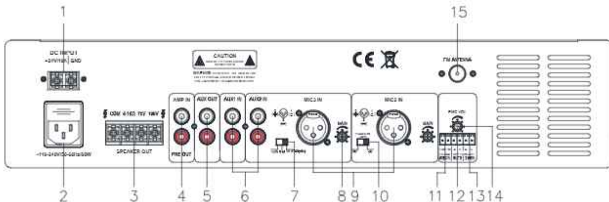
DMA250U Rear Panel
