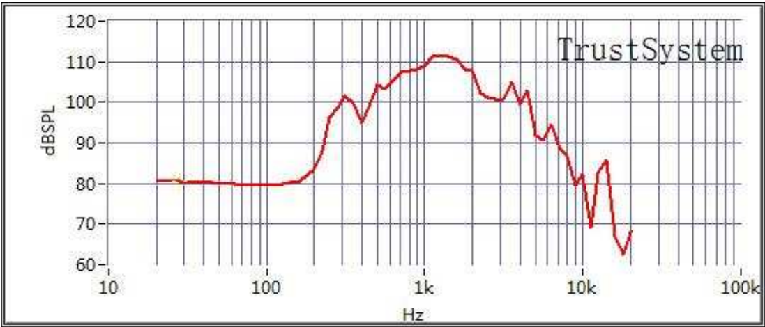
Frequency Response @ /1W/1m
