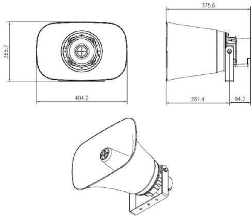
Dimension Diagram
